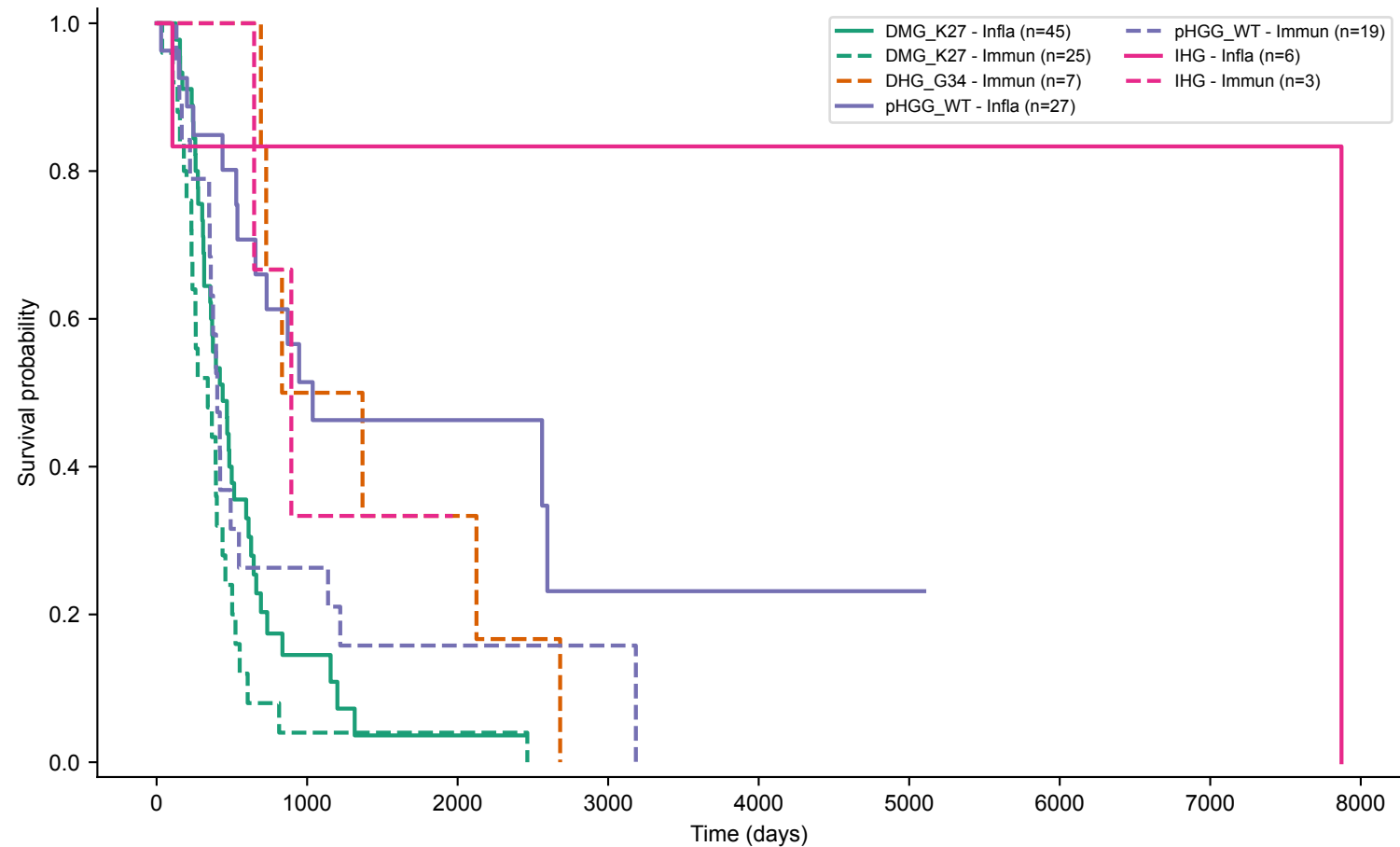
Kaplan-Meier by ecotype within each cohort group (solid = Inflamed, dashed = Immune-desert)
